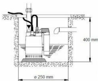
With vertical level switch
