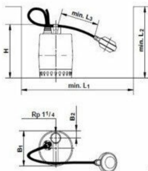
With float switch
